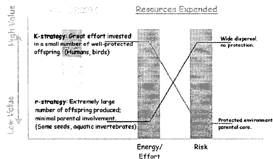
Figure 5 - r & K scenario logic
