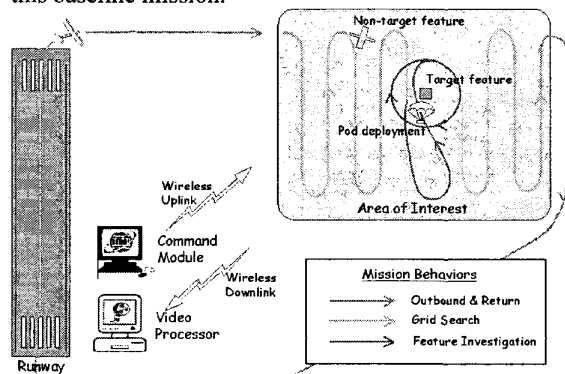
Figure 11– Schematic of 10/02 Baseline Flight Demo
